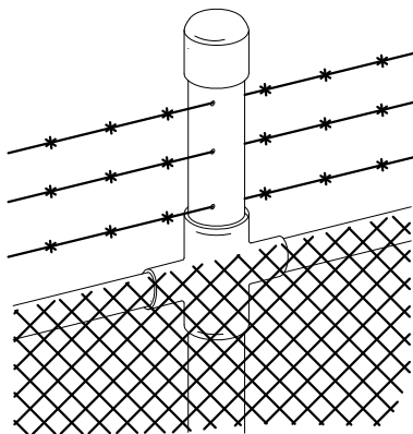
EXTENSION POST AND BARBED WIRE DETAIL NO SCALE
